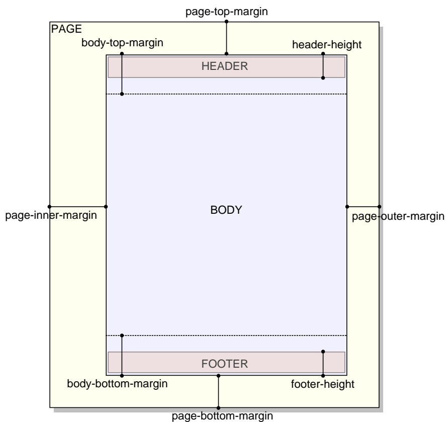
Figure 10-1. Page areas
